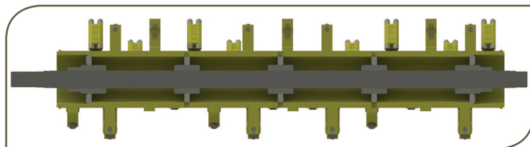
Heavy duty rotor construction; balanced .75" wall drum with 2.438" alloy steel shaft through entire length of rotor; new rotor spiral cut pattern cuts the entire length of rotor and reduces the amount of cut per tooth maximizing efficiency
