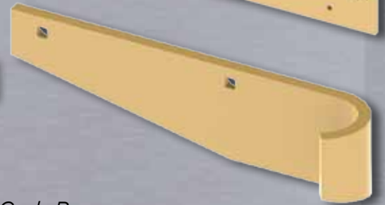
Curb Bumper Wraps around end of blade, useful for protecting outside edge of plow and blade bottom edge. Also used to prevent leading edge of JOMA blade from catching in roadway obstructions ie. Bridge joints, railway crossings etc. Bolts over clamping bar.
